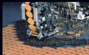
Sequin Device IV A device for embroidering various sequins: small-diameter sequins, large-diameter sequins, irregular-shape sequins and eccentric sequins
